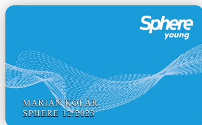
SPHERE YOUNG
