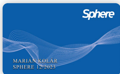
SPHERE
